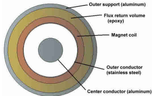
Figure 1. Magnetically-insulated transmission line, outer diameter 7.6 cm
