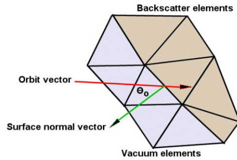
Figure 2. Representing backscatter on a conformal mesh
