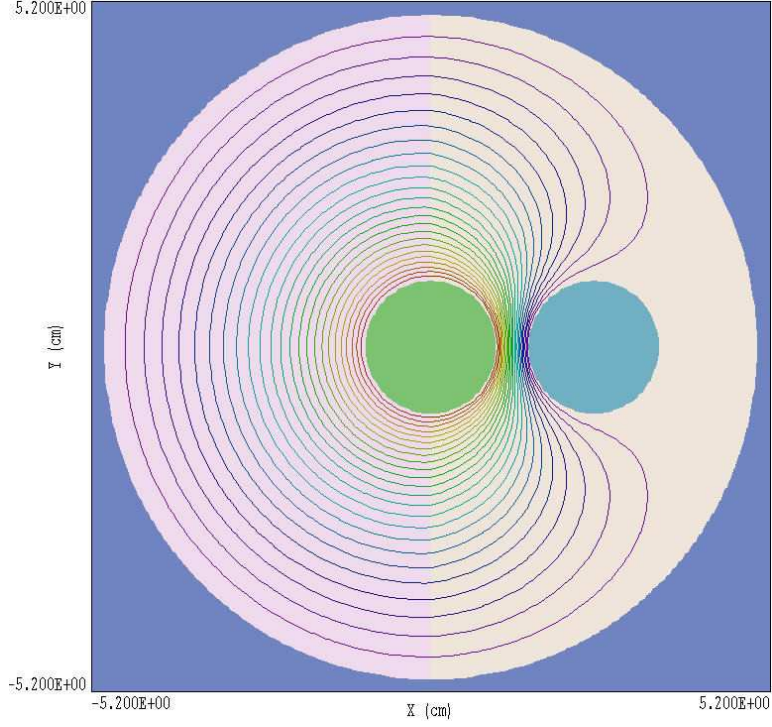
Figure 2: Calculated equipotential lines for Solution 1.
