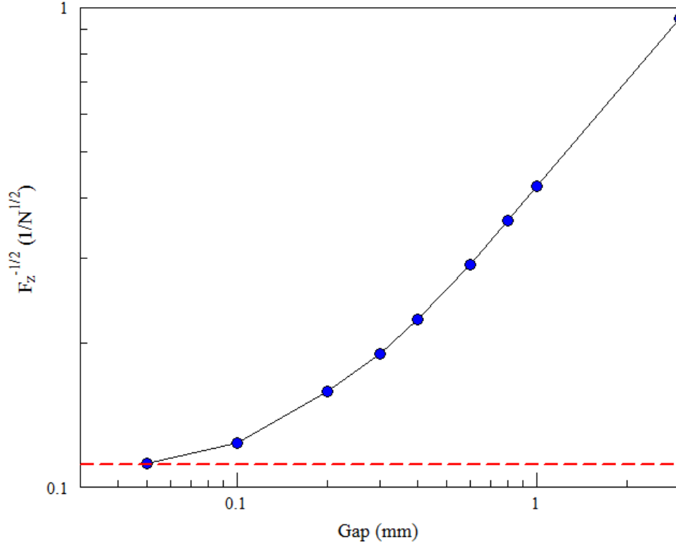
Figure 4: Plot of F_z^{-1/2} as function of the gap between the plunger and the bobbin, where F_z is the force on the plunger in newtons. Blue circles indicate results determined by a surface integral in MagView . The dashed red line indicates the theoretical value for zero gap.
