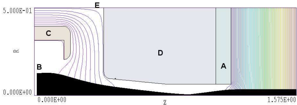
Figure 2: Electron gun concept, showing equipotential lines and electron orbits for I_b = 80.0 mA, accelerator phase 90^\circ . A ) Accelerator entrance flange and aperture (see Fig. 1). B ) Control grid surface. C ) Grid support extension. D ) Anode. E ) Vacuum chamber inner wall. (Dimensions in inches.)
