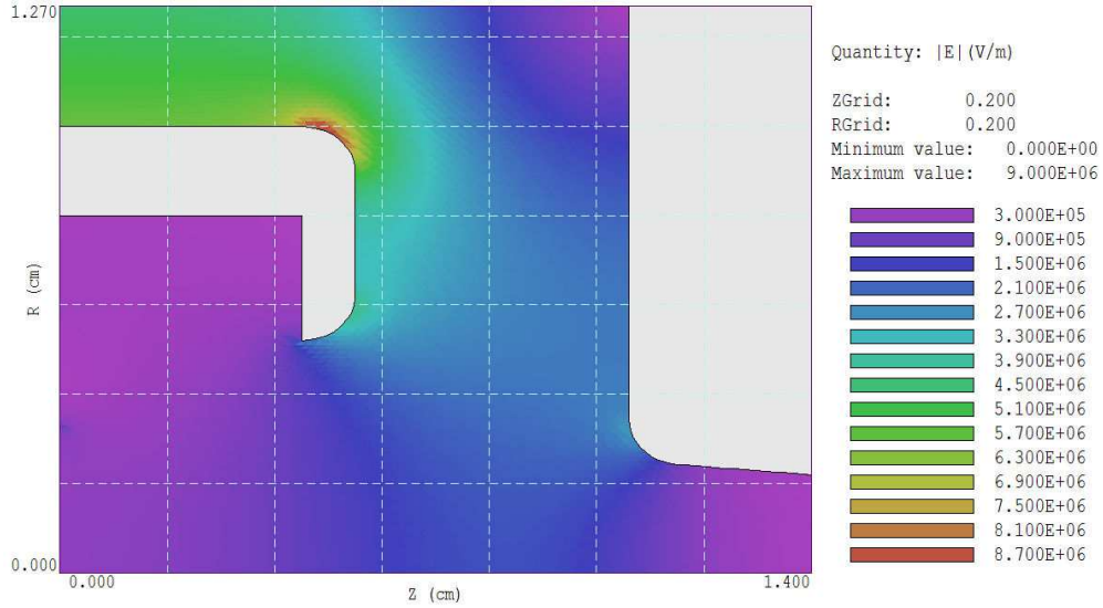
Figure 5: Map of |\mathbf{E}| in the electron gun. (Dimensions in cm.)
