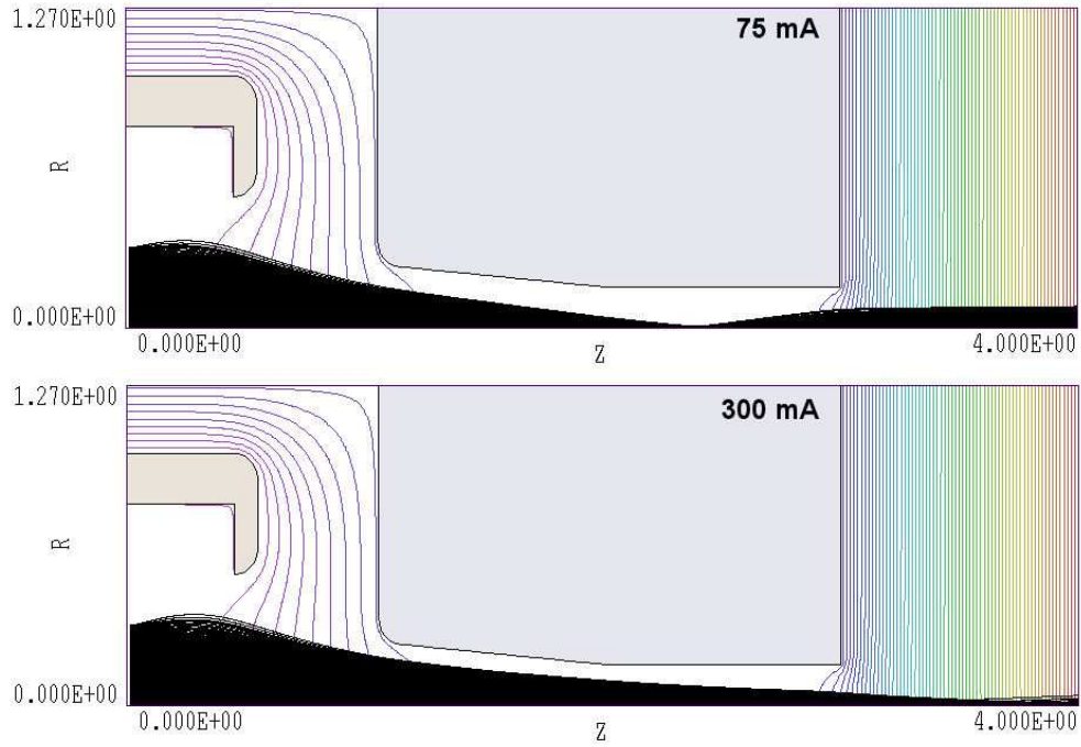
Figure 3: Beam profile at two current levels, accelerator phase 90^\circ . Top: 75.0 mA. Bottom: 300.0 mA. (Dimensions in cm.)
