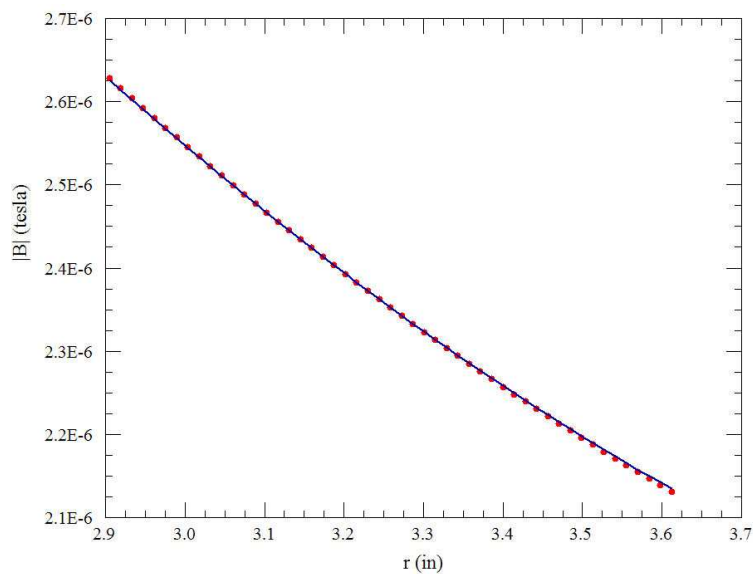
Figure 4: Plot of |B| as a function of r along a 45^\circ line for a highly elliptical center conductor (BDOT05). Solid line: z = 0.000 ". Symbols: z = 0.340 ".
